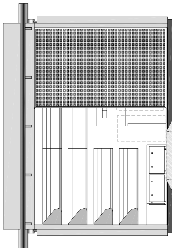
VISTA 2 – LAYOUT
